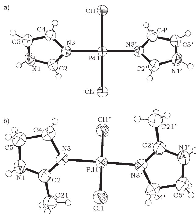
Figure 1. X-ray structures of the PdCl 2 – 1a complex (above) and the PdCl 2 – 1e complex (below).
