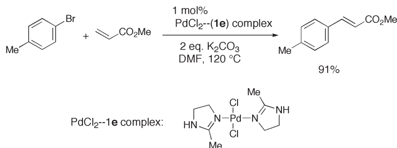
Scheme 1. Mizoroki–Heck reactions between 4-bromotoluene and methyl acrylate in the presence of PdCl 2 – 1e complex.
